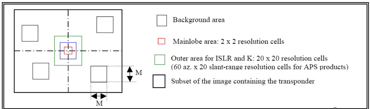
Figure 1 Definition of point target response area and background areas for IRF analysis and calibration.
