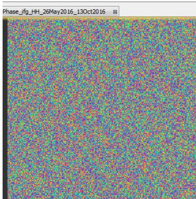
interferogram generated
