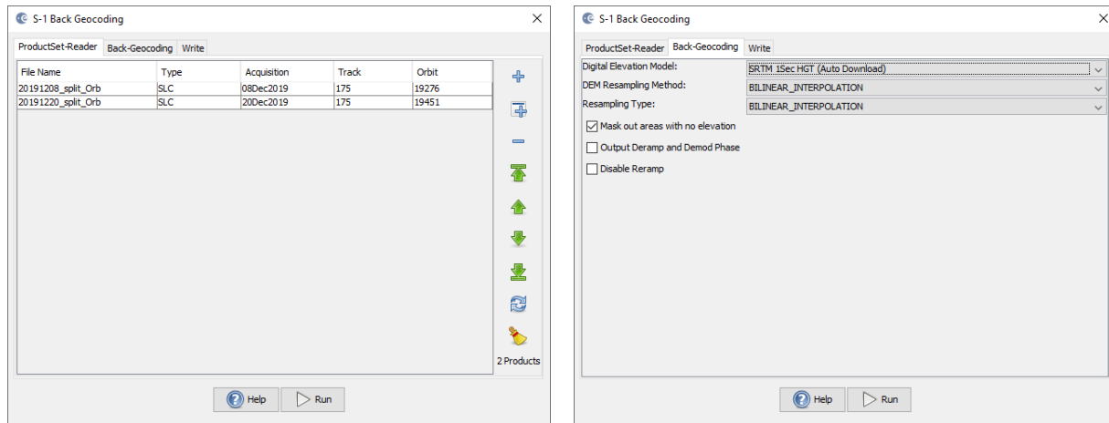
Figure 9: Back Geocoding
