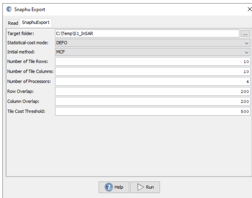
Figure 20: Snaphu export
