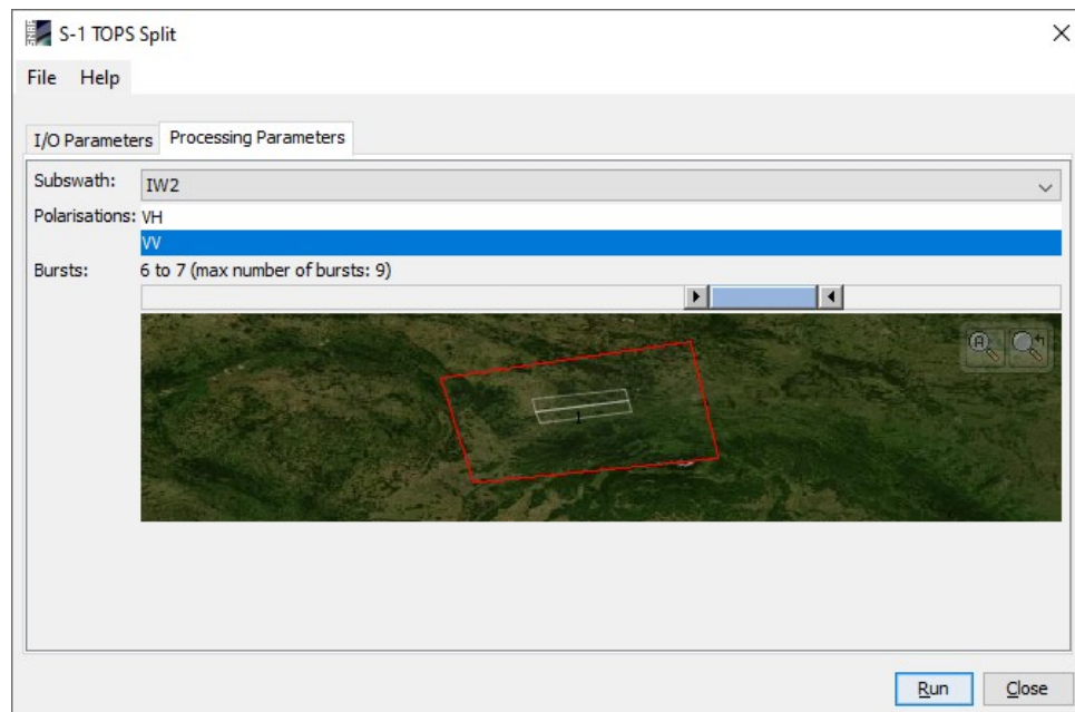
Figure 7: TOPS Split
